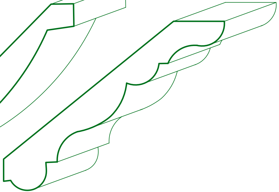
MC - 3003 25/32" x 4 15/16"
