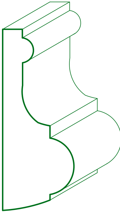
MC - 3823 1 5/16 X 3 5/16
