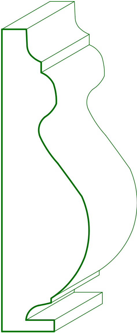
MC - 260 Plinth Block 1 1/2 X 5 5/32
