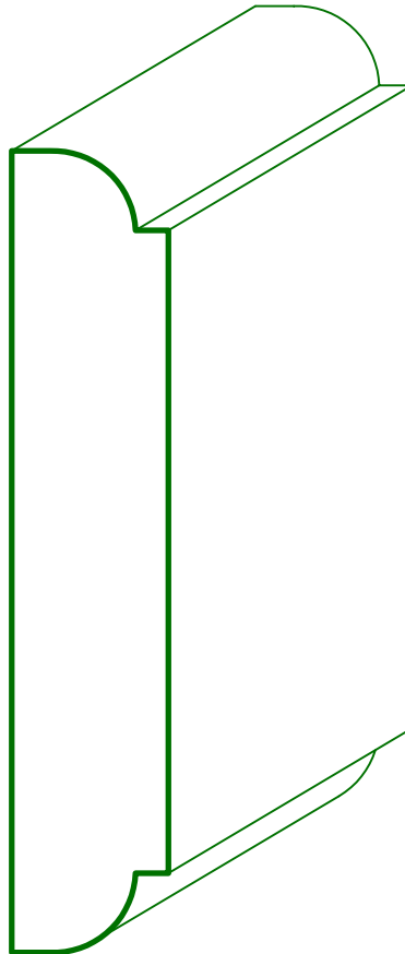
MC-505 3/4 X 4 1/4 3/4 X 4 1/2 3/4 X 4 3/4
