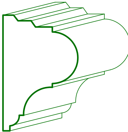
MC-225 1 3/8 X 2
