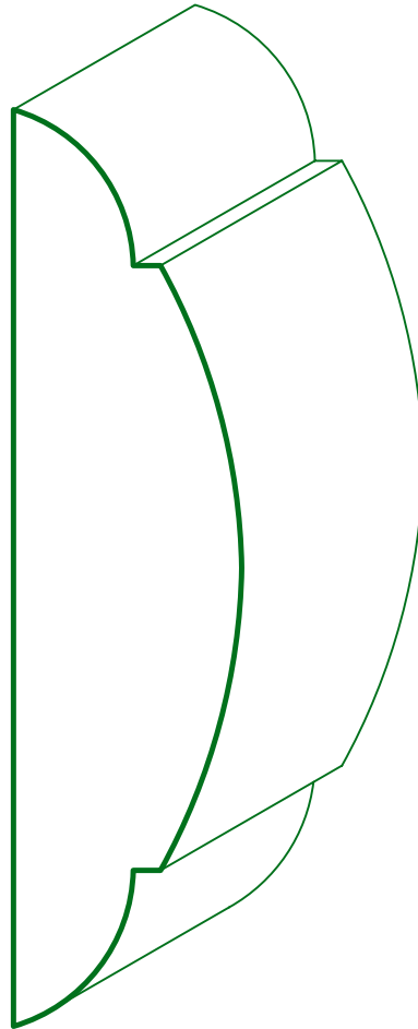
MC - 3062 1 1/16" x 4 3/8"
