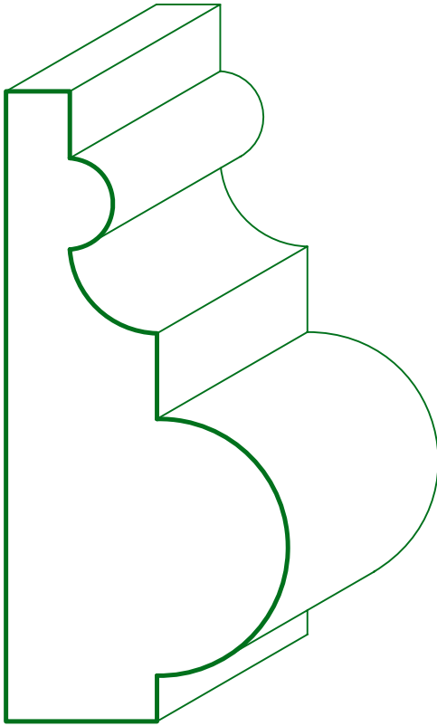
MC - 3220 1 5/8" x 3 5/8"
