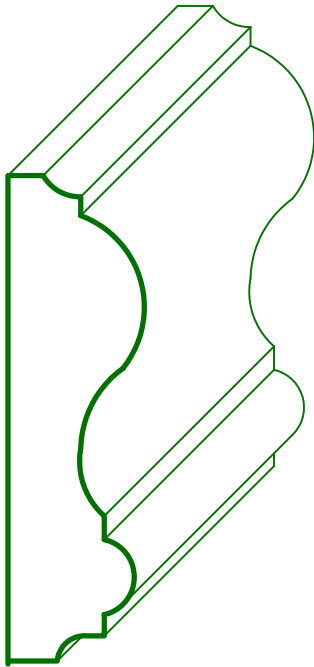
MC - 40 3/4 x 2 1/2
