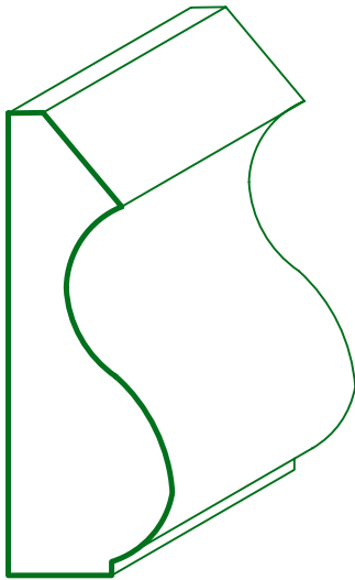
MC - 2939 3/4" x 2 3/16"
