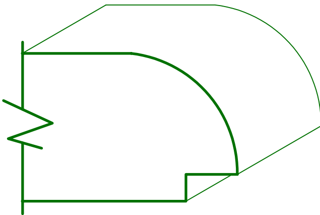
MC-358 1 1/2 X WIDTH
