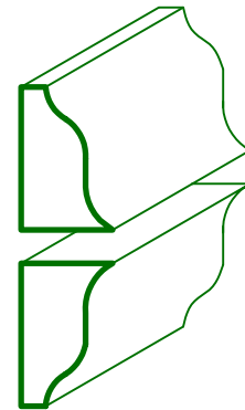
MC - 1066 SPLITTER 7/16 X 11/16
