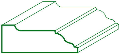
MC - 4013 19/32 X 1 19/32
