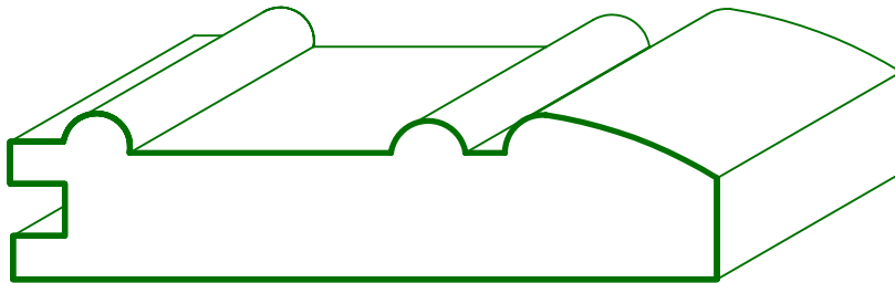
MC - 1164 3/4 X 3 5/16
