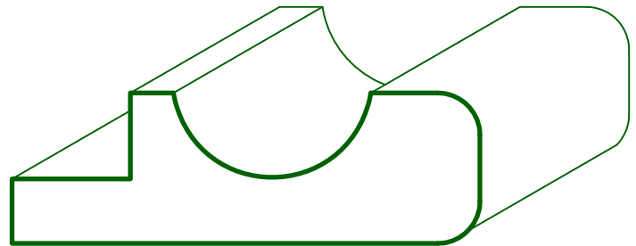
MC 4024 7/8 x 2 23/32
