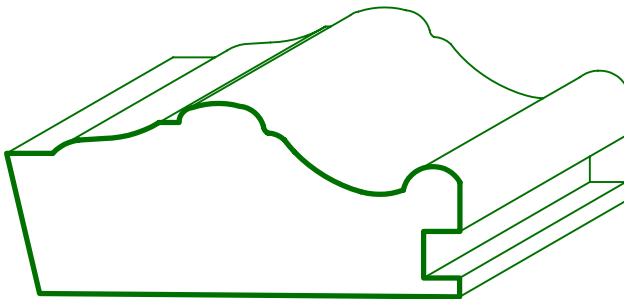
MC 2495 1" x 2 3/8"
