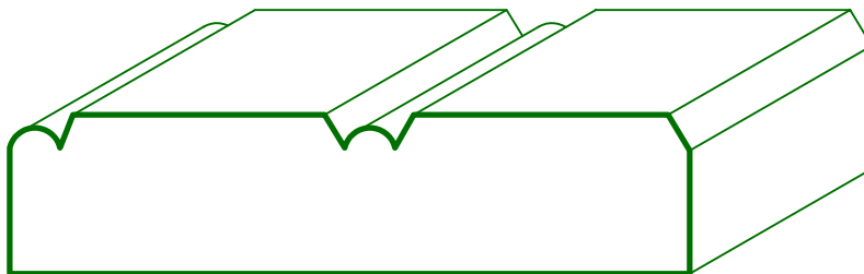
MC-238 3/4 X 3 1/4
