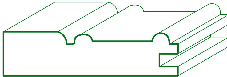
MC - 3842 3/4 X 2 15/16
