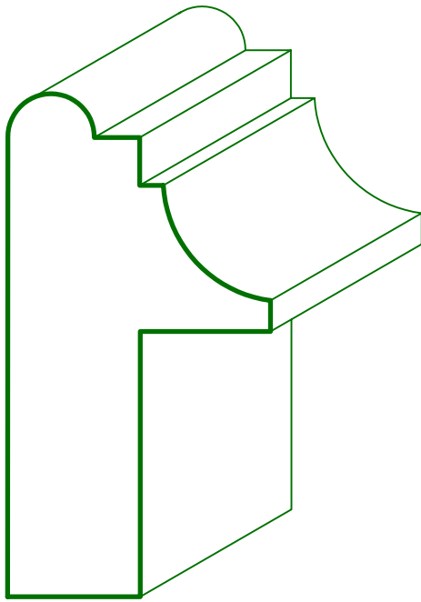
MC - 1756 1 1/2 X 2 7/8
