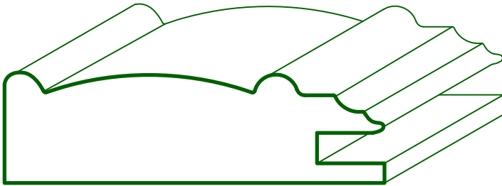
MC 4170 25/32 x 2 3/4
