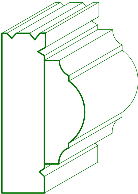
MC - 776 775 7/8 X 3 5/16
