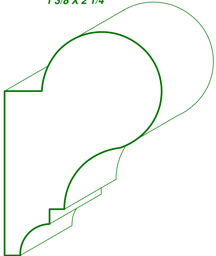
MC - 1907 2 5/8 X 3 3/4
