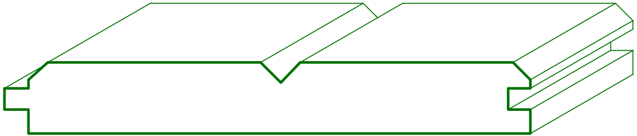
MC-76 3/4 X 5 1/2
