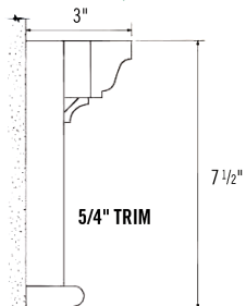
Window/Door Header
