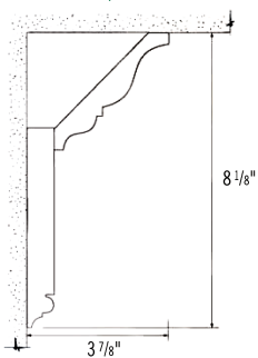
Crown/Cornice
